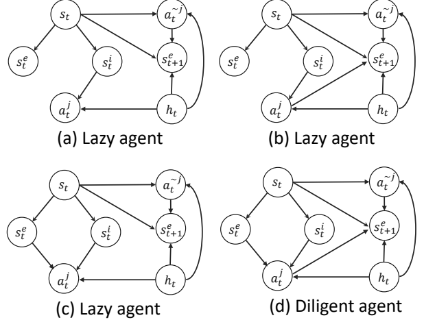
Figure 2. Causal diagrams of three types of lazy agents and diligent agent. We mainly consider agent j here. h_t is the historical state trajectory information. a_t^{\sim j} is joint action except for agent j .
