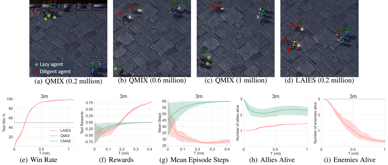
Figure 1. (a), (b) and (c) depict the policies obtained by QMIX after 0.2 million steps, 0.6 million steps, and 1 million steps of training respectively, under the condition of sparse rewards. (d) illustrates the policy obtained by LAIES after 0.2 million steps of training. The green and red points label lazy agents and diligent agents, respectively. The curves in (e) - (i) represent the average test results of five different random seeds.
