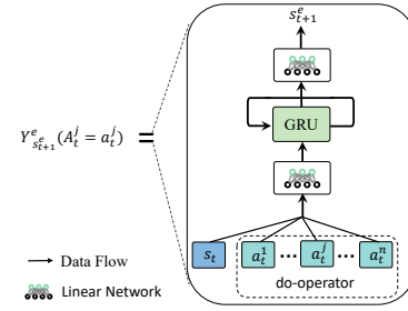
Figure 3. Network architecture of ESTM. GRU is used to capture historical information.
