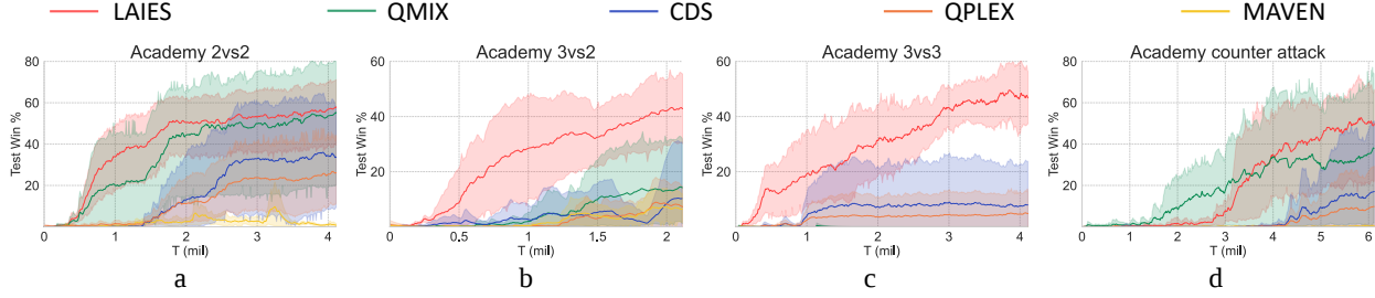
Figure 5. Comparison of our method against baseline methods on four tasks in GRF with the evaluation index of test winning rate.
