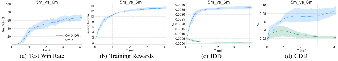
Figure 7. Experimental results on 5m_vs_6m task in SMAC. Figures (c) and (d) are the change curve of IDD and CDD of QMIX and QMIX-DR during training.
