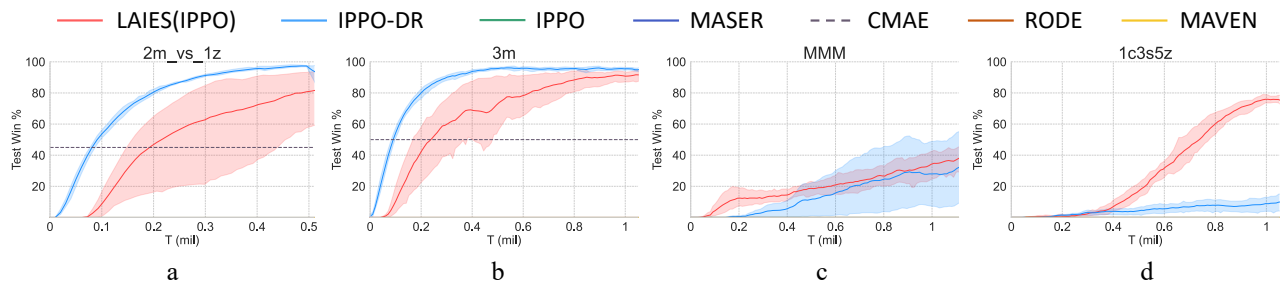
Figure 9. Comparison of our method against baseline methods on four tasks in SMAC with the evaluation index of test winning rate.
