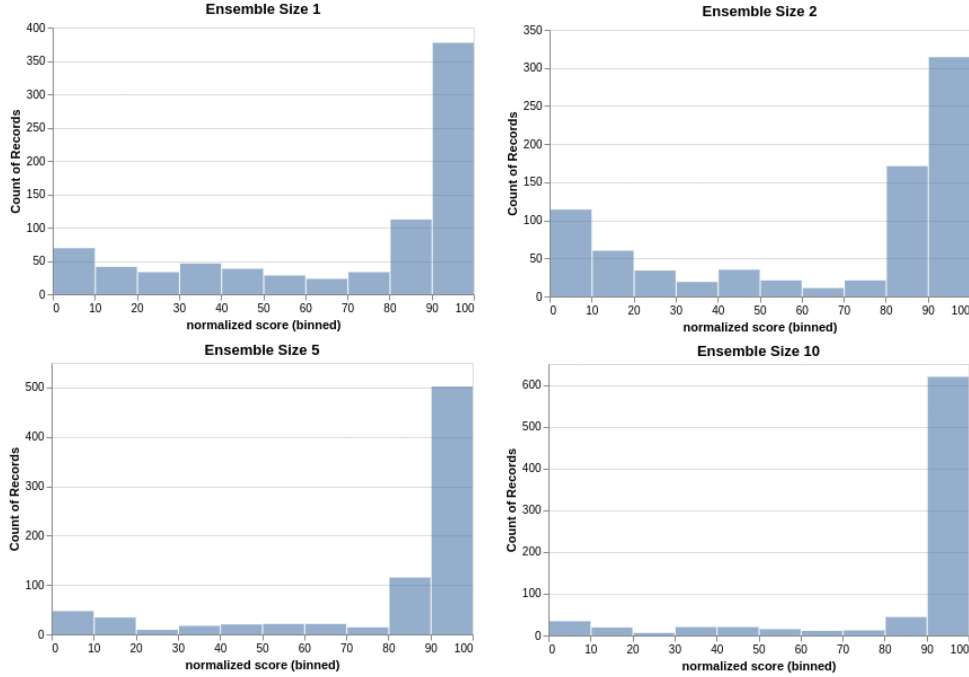
Figure 8: Performance of \mathcal{L}_{MG} with varying ensemble sizes on Walker2d-Medium-Replay-v2. Each variant aggregates returns over 8 seeds, and each seed evaluates for 100 episodes. Each Q -value network is modeled by a 3-layer MLP. With lower ensemble size, the performance exhibits large variance across different episodes.
