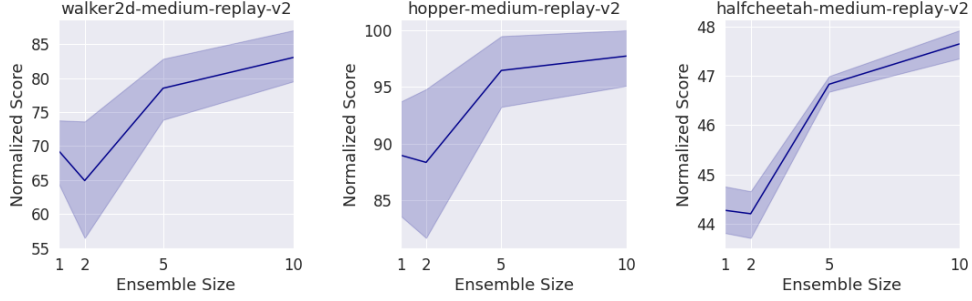
Figure 7: Performance of \mathcal{L}_{MG} with varying ensemble sizes. Each variant averages returns over 8 seeds, and each seed contains 100 evaluation episode. Each Q -value network is modeled by a 3-layer MLP. The shaded area denotes bootstrapped 95% CI.
