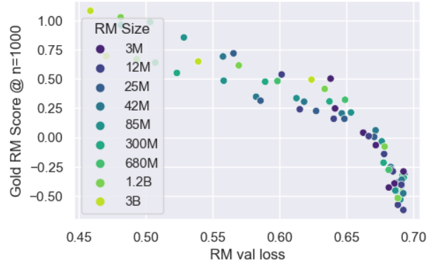
Figure 7: RM validation loss vs BoN RM score @ n=1000. Most points in this figure are already averaged over multiple seeds.
