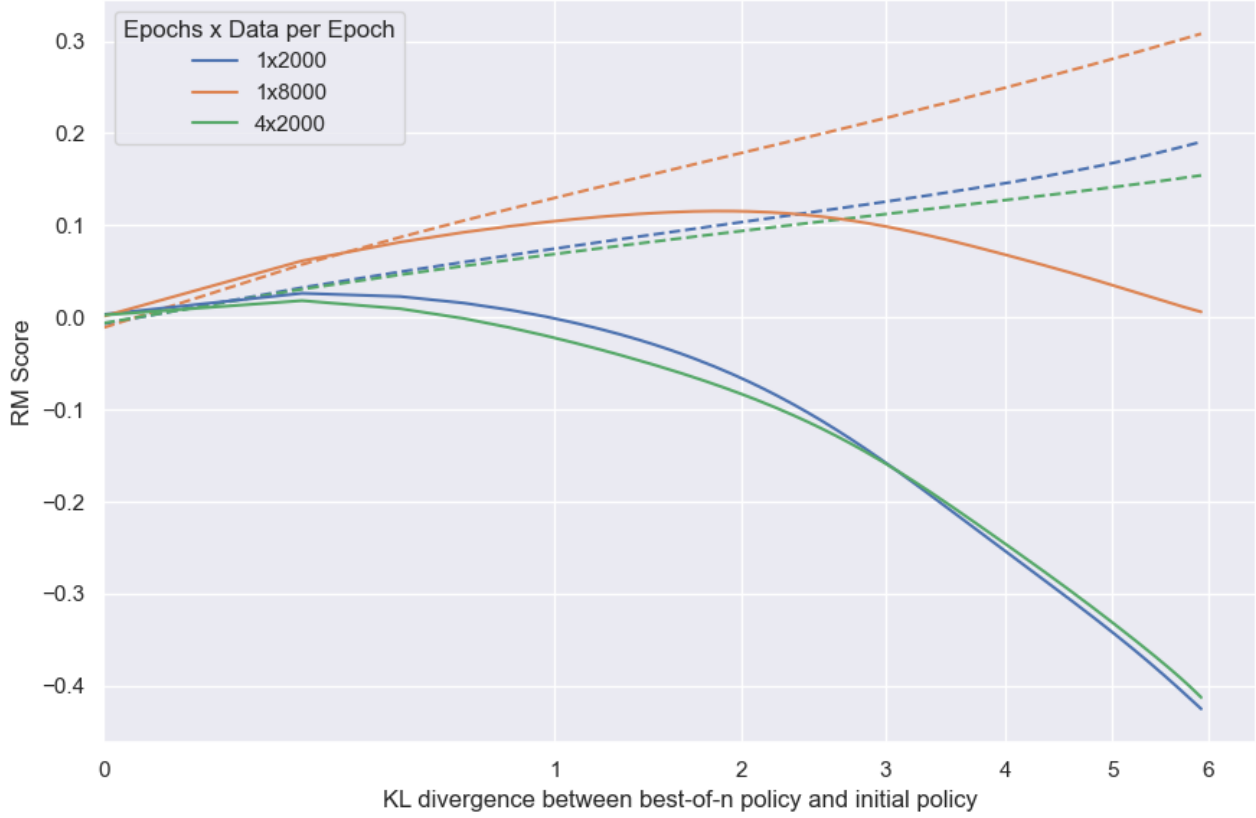
Figure 13: Total number of data points seen does not seem to affect the gold RM score much compared to the number of unique data points seen. Averaged across RM sizes. The numbers of datapoints (2000–8000) is intentionally chosen to straddle the sharp increase in performance. The validation loss of the 1x2000, 1x8000, and 4x2000 RMs are 0.686109, 0.654857, and 0.683869 respectively.
