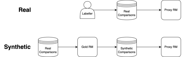
Figure 1: Diagram of the real and synthetic Reward Model (RM) training setups. Human labellers generate comparison data. In the real RLHF setting, this data is used to train a proxy RM that is optimized by RL/BoN. In our synthetic setting, we instead use a “Gold RM” as our ground truth. In both settings, the proxy RM is a proxy for the ground truth process generating the labels (either the human or gold RM).
