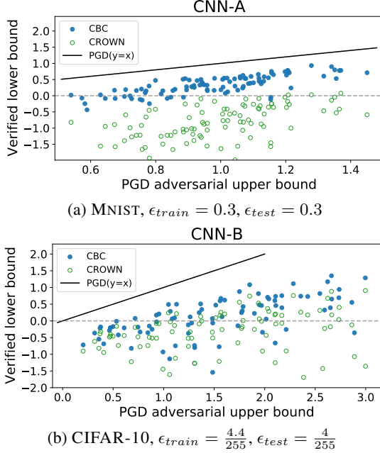
Figure 6. Comparing the tightness of verifiers. For 100 test samples on MNIST and CIFAR-10. (a) runs on CNN-A, (b) runs on CNN-B. We plot the verified lower bound \underline{f}(x^+, x^-, \epsilon) against PGD upper bound \bar{f} . Some points exceed the plotted axes limits.
