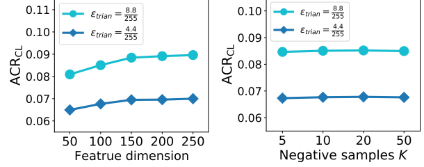
Figure 7. Left: Sensitivity analysis of feature dimension influencing \text{ACR}_{\text{CL}} . Right: Sensitivity analysis of the number of negative samples K influencing \text{ACR}_{\text{CL}} . Experiments run on CNN-B with different \epsilon_{\text{train}} on CIFAR-10.
