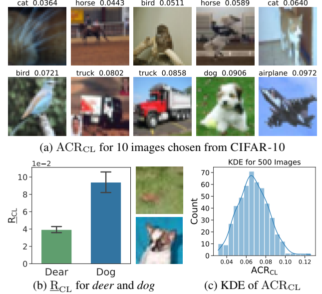
Figure 5. (a,b,c) run on CNN-B with \epsilon_{train} = 4.4/255 . (a) ACR_{CL} for images, which are randomly chosen from CIFAR-10; K = 50 . (b) \underline{R}_{CL} for two images from CIFAR-10; K = 50 . (c) Frequency distribution histogram and kernel density estimation (KDE) of ACR_{CL} for 500 images from CIFAR-10; K = 20 .
