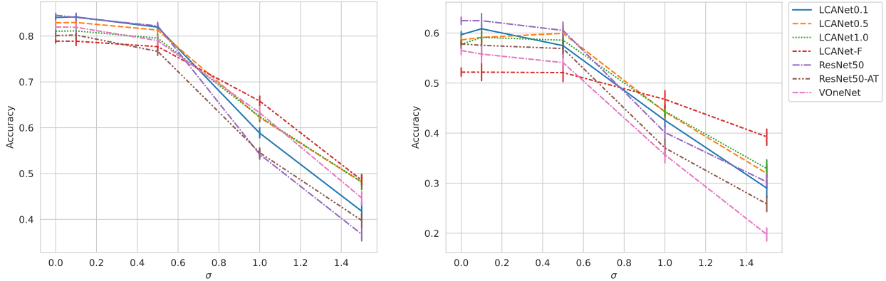
Figure 3. LCA-Nets are more robust to Gaussian blurring than state-of-the-art robust models. Although accuracy decreases uniformly over all models on the UCF-101 (left) and HMDB-51 (right) datasets, LCA-Nets maintain a small gain in accuracy over robust models under increased blurring. Strikingly, the unsupervised LCA features exhibit the most robustness of all models tested, as the LCA-Nets-F model outperforms or matches the second most robust model on this corruption.
