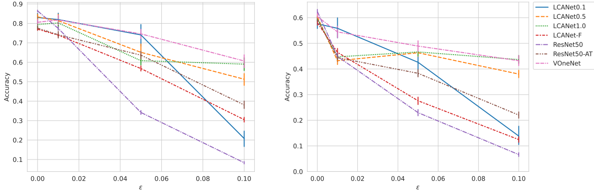
Figure 4. LCA N ets are as robust to high strength black-box attack as state-of-the-art defense methods. Although VOne N ets are the most robust on average over all three attack strengths of this L_\infty constrained black-box attack (Ilyas et al., 2018), LCA N ets perform about the same or only a few percentage points worse while also outperforming adversarially trained Res N ets on UCF-101 (left) and HMDB-51 (right).
