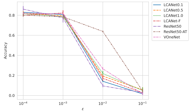
Figure 5. LCA N ets are susceptible to white-box attacks. Here, we see that the adversarially-trained CNN (Res N et50-AT) performs significantly better under a PGD attack than all other models on the UCF-101 dataset, which is to be expected. Although the LCA N ets are not nearly as robust as the adversarially-trained CNN, they are still significantly more robust than a standard CNN.
