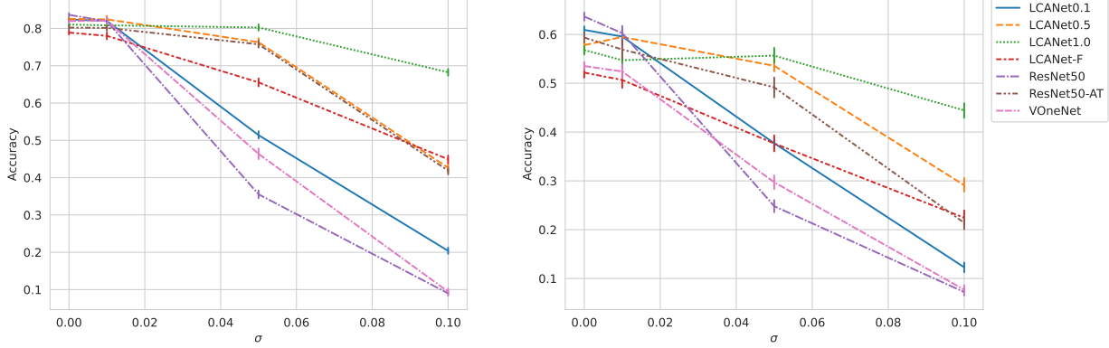
Figure 2. LCA-Nets are significantly more robust to Gaussian noise than state-of-the-art robust models. LCA-Nets significantly outperform all other models under additive Gaussian noise on both the UCF-101 (left) and HMDB-51 (right) datasets. The unsupervised LCA features appear to contribute significantly to this robustness, as indicated by the moderate robustness exhibited by LCA-Nets-F.
