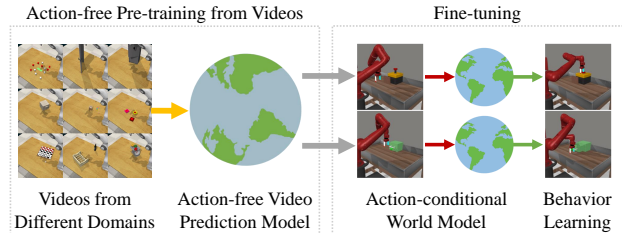
Figure 1. We pre-train an action-free latent video prediction model using videos from different domains (left), and then fine-tune the pre-trained model on target domains (right).
