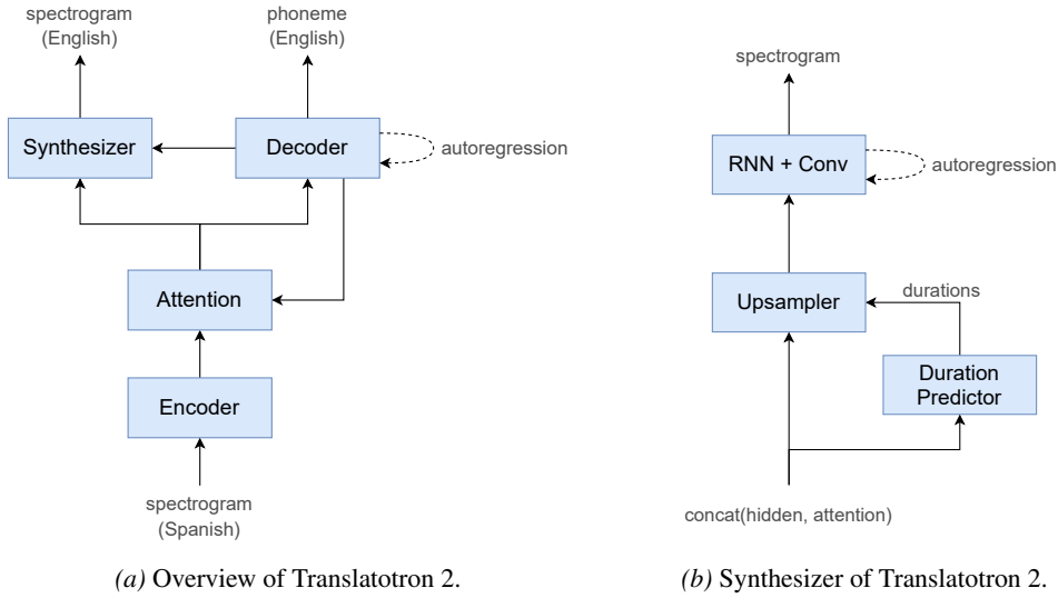
Figure 1: A Translatotron 2 model that translates Spanish speech into English speech.
