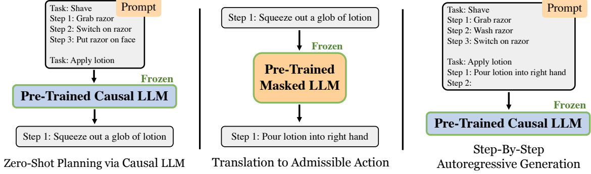
Figure 3. We first show surprising finding that pre-trained causal LLMs can decompose high-level tasks into sensible mid-level action plans ( left ). To make the plans executable, we propose to translate each step into admissible action via another pre-trained masked LLM ( middle ). The translated action is appended to the prompt used for generating the remaining steps ( right ). All models are kept frozen without additional training.
