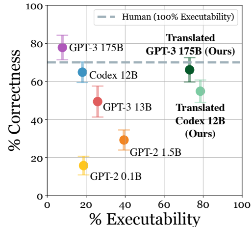
Figure 1. Executability (x-axis) and semantic correctness (y-axis) of generated action plans. Large models can produce plans indistinguishable from those by humans, but frequently are not executable in the environment. Using our techniques, executability is significantly improved, albeit at the cost of correctness. Website: https://huangwl18.github.io/language-planner/ .
