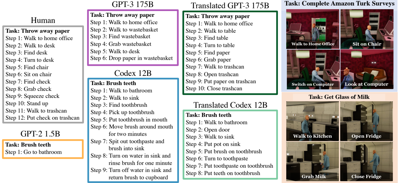
Figure 2. Sample action plans generated by different models (left) and visualization of VirtualHome execution of plans generated by our approach (right). We show LLMs not only can generate sensible action plans given only high-level tasks but also contains the actionable knowledge that can be extracted to perform common-sense grounding in embodied environments. More samples in Appendix A.7.
