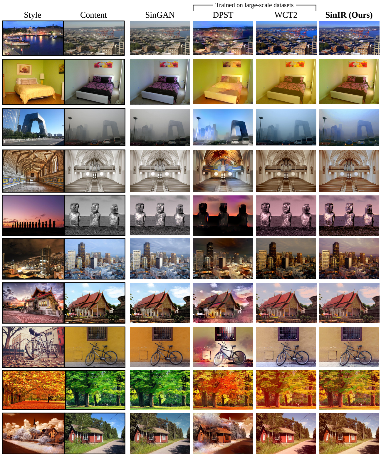
Figure 2. Photo-realistic Style Transfer. DPST (Luan et al., 2017) and WCT2 (Yoo et al., 2019) are dedicated methods.
