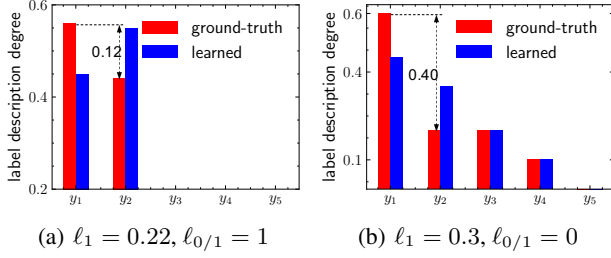
Figure 2. Illustration of objective mismatch. The red and blue bars are the ground-truth the learned label distributions, respectively. Fig. 2(a) has a lower L_1 -norm loss than Fig. 2(b), while Fig. 2(b) has a lower 0/1 loss than Fig. 2(a). Note that Fig. 2(a) is superior to Fig. 2(b) in terms of LDL and inferior to Fig. 2(b) in terms of classification, which justifies the objective mismatch.
