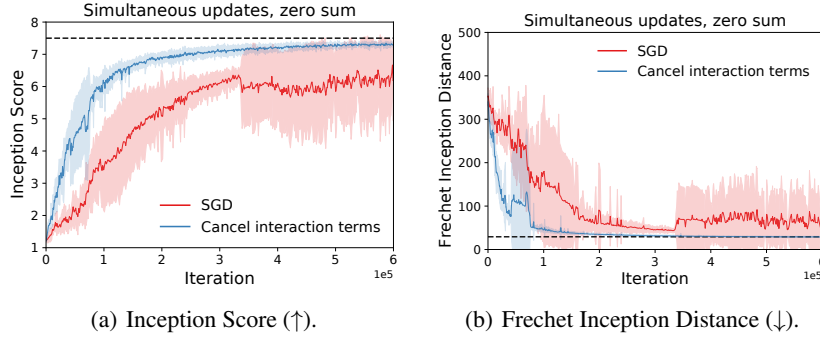
Figure A.6. Using explicit regularization to cancel the effect of the interaction components of drift eads to a substantial improvement compared to SGD without explicit regularization.
