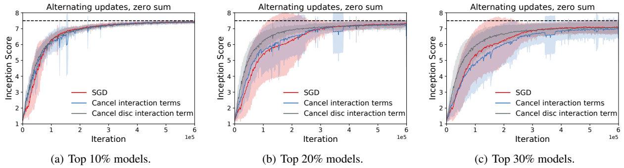
Figure A.19. Performance across the top performing models for vanilla SGD and with canceling the interaction terms and only cancelling the discriminator interaction terms. We notice that canceling only the discriminator interaction terms can result in higher performance across more models, and that the interaction term of the generator can play a positive role, likely due to the smaller strength of the generator interaction term compared to simultaneous updates.
