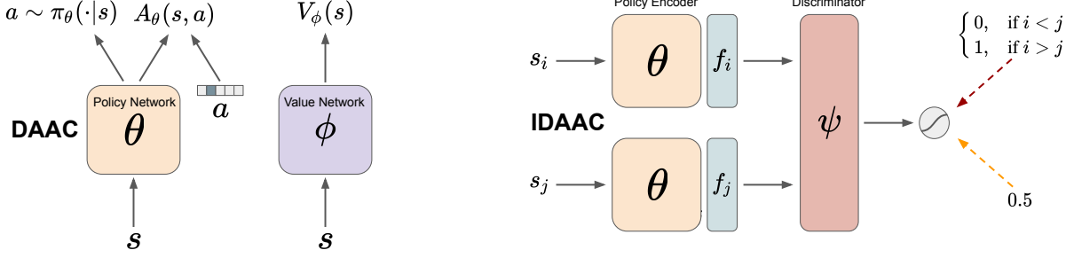
Figure 2. Overview of DAAC (left) and IDAAC (right). DAAC uses two separate networks, one for learning the policy and advantage, and one for learning the value. The value estimates are used to compute the advantage targets. IDAAC adds an additional regularizer to the DAAC policy encoder to ensure that it does not contain episode-specific information. The encoder is trained adversarially with a discriminator so that it cannot classify which observation from a given pair (s_i, s_j) was first in a trajectory.
