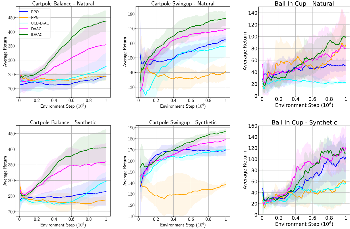
Figure 11. Average return on three DMC tasks, Cartpole Balance (left), Cartpole Swingup (center), and Ball In Cup (right), with natural (top) and synthetic (bottom) video backgrounds. The mean and standard deviation are computed over 10 runs with different seeds. DAAC and IDAAC outperform PPO, PPG, and UCB-DrAC.
