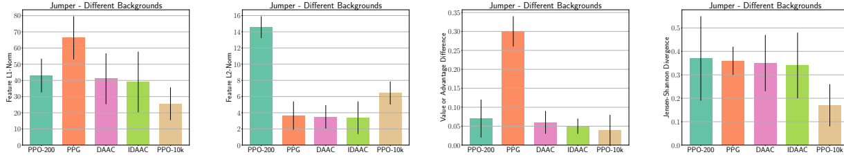
Figure 22. Variations in the learned features, policies, and values or advantages when changing the background in Jumper. From left to right we report the L1 and L2-norm for the features, the value or advantage difference, and the Jensen-Shannon Divergence for the policy. We compare PPO trained on 200 and 10k levels with PPG, DAAC, and IDAAC. Our models are more robust to changes in the background (which does not affect the state). The means and standard deviations were computed over 10 different backgrounds.
