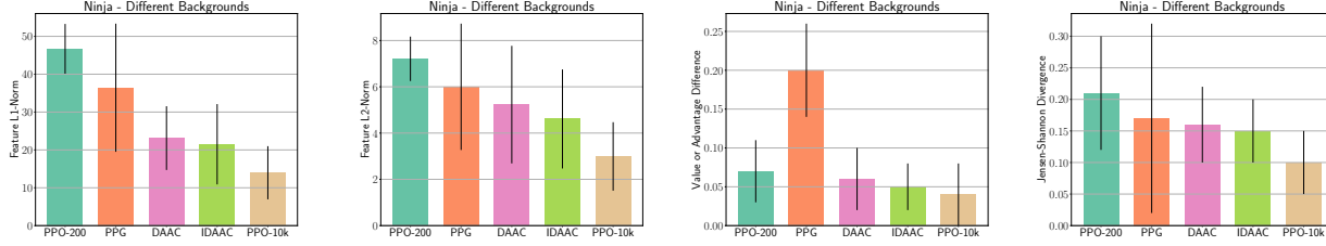
Figure 21. Variations in the learned features, policies, and values or advantages when changing the background in Ninja. From left to right we report the L1 and L2-norm for the features, the value or advantage difference, and the Jensen-Shannon Divergence for the policy. We compare PPO trained on 200 and 10k levels with PPG, DAAC, and IDAAC. Our models are more robust to changes in the background (which does not affect the state). The means and standard deviations were computed over 10 different backgrounds.
