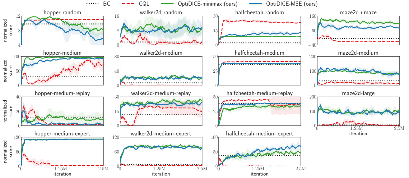
Figure 9. Performance of BC, CQL, OptiDICE-minimax and OptiDICE-MSE on D4RL benchmark for \gamma = 0.999 .
