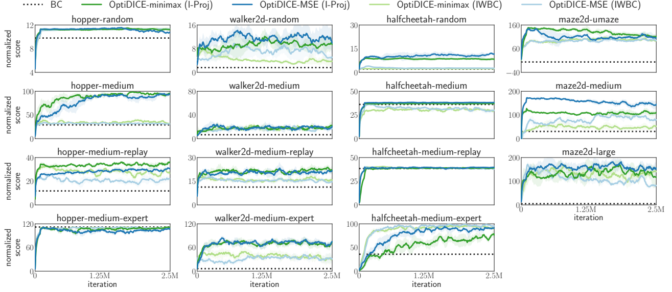
Figure 7. Performance of BC, OptiDICE with importance-weighted BC (IWBC) and information projection (I-Proj) methods on D4RL benchmark. \gamma = 0.99 is used.
