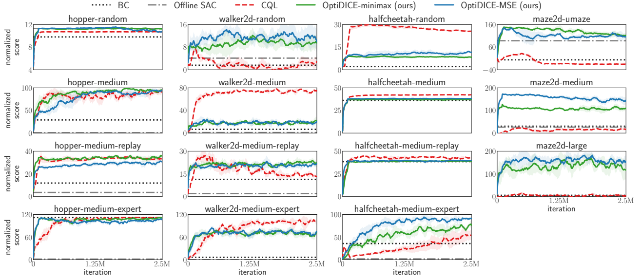
Figure 8. Performance of BC, CQL, OptiDICE-minimax and OptiDICE-MSE on D4RL benchmark for \gamma = 0.99 .
