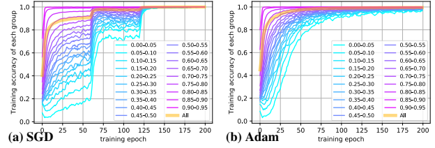
Figure 10. Learning speed of CIFAR-10 examples grouped by C-score. The thick transparent curve shows the average accuracy over the entire training set. SGD achieves test accuracy 95.14%, Adam achieves 92.97%.
