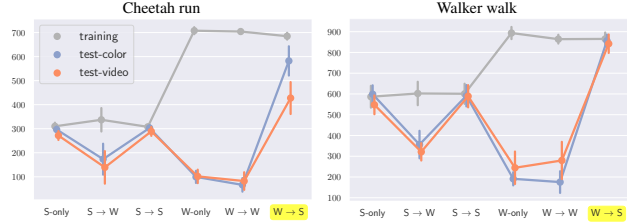
Figure 3. Ablation on different strategies to apply augmentation. “S-only” denotes single-stage policy trained with strong augmentation, and S → W means strongly-augmented expert imitated by weakly-augmented student. The recipe for SECANT is W → S .
