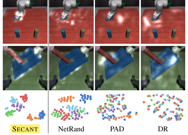
Figure 4. Row 1 and 2: saliency map of the learned policies in unseen tests. SECANT attends to the components crucial to the task, while other agents often focus on irrelevant places. Row 3: t-SNE visualization of state embeddings. Our method correctly groups semantically similar states with different visual appearances.
