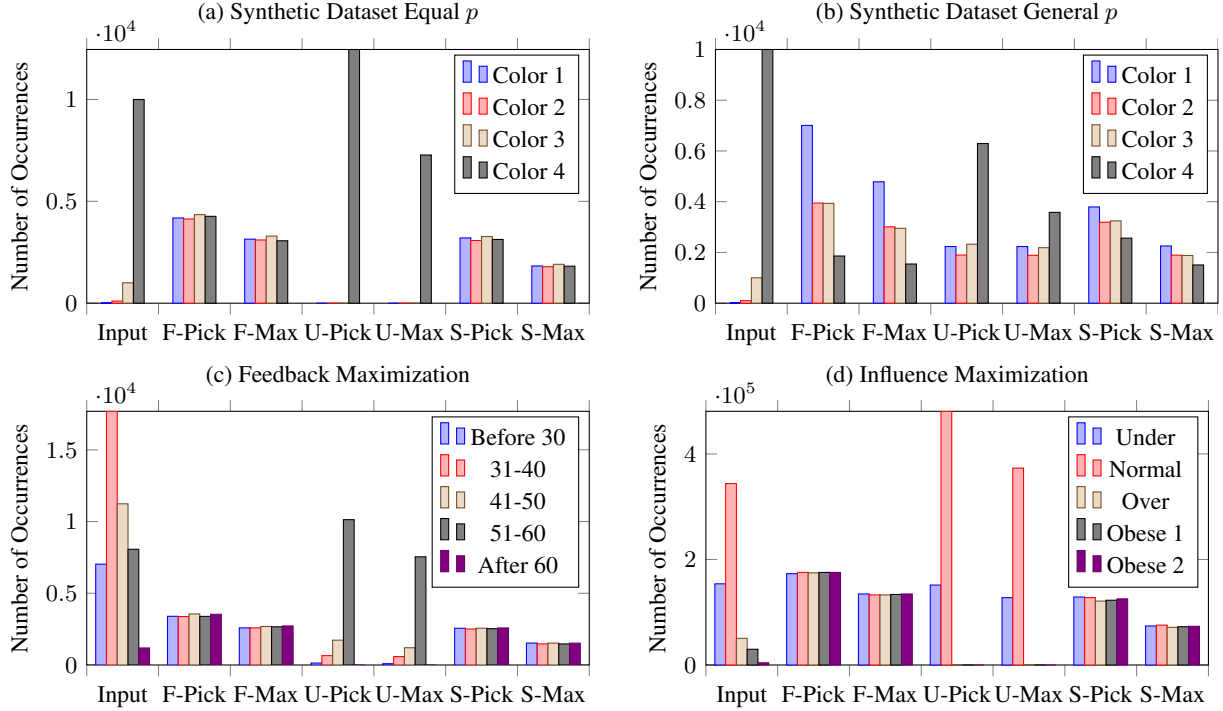
Figure 1. In this plot, we compare our fair secretary algorithm with the secretary algorithm (SA) and the single-color secretary algorithm (SCSA) on (a) synthetic dataset, equal \mathbf{p} values, (b) synthetic dataset, general \mathbf{p} values, (c) feedback maximization dataset, and (d) influence maximization dataset. Here Input is the number of elements from each color in the input, F-Pick and F-Max are the number of elements picked by our fair secretary algorithm and the number of them that are the maximum among the elements of that color. Similarly, U-Pick (S-Pick) and U-Max (S-Max) are the number of elements picked by SA and SCSA and the number of them that are the maximum among the elements of that color.
