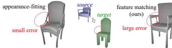
Figure 1. Limitation of global shape error metrics. Mesh deformed from source (blue) to target (green). The appearance-fitting result, generated with MeshODE (Huang et al., 2020), has a lower global matching error from the target shape at the arms (e.g. Chamfer distance), with an unnatural fitting.
