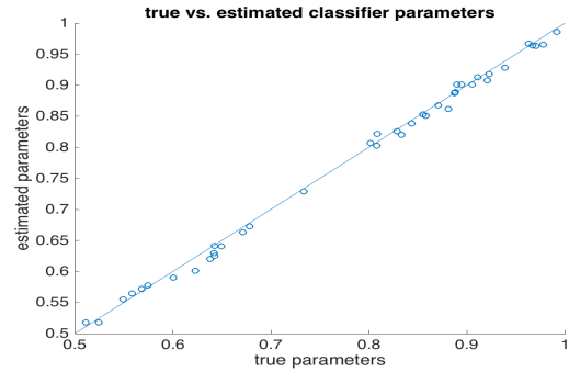
Figure 5. Recovery of the conditional Independence model parameters \{\psi_i, \eta_i\} from a RBM with a single hidden node, on a dataset sampled from a conditional independence model. The parameters were uniformly sampled from [0.5, 1] . Each circle corresponds to a single parameter (e.g., \psi_i for some i ). For convenience, the identity line was added to the plot.
