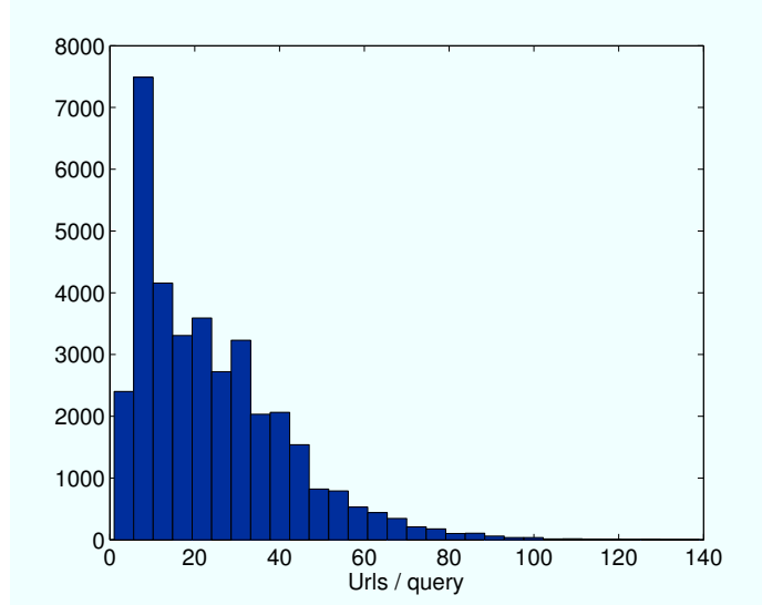
Figure 1: Distribution, over both sets, of the number of documents per query.
